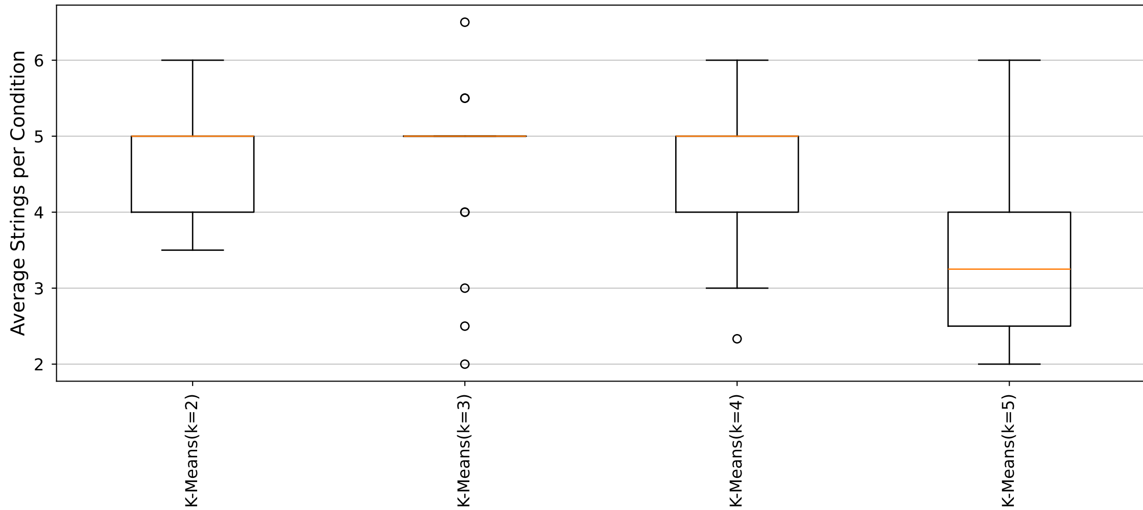
YARA Rules Average Strings per Condition Distribution (Cluster36_Size5 dataset)
